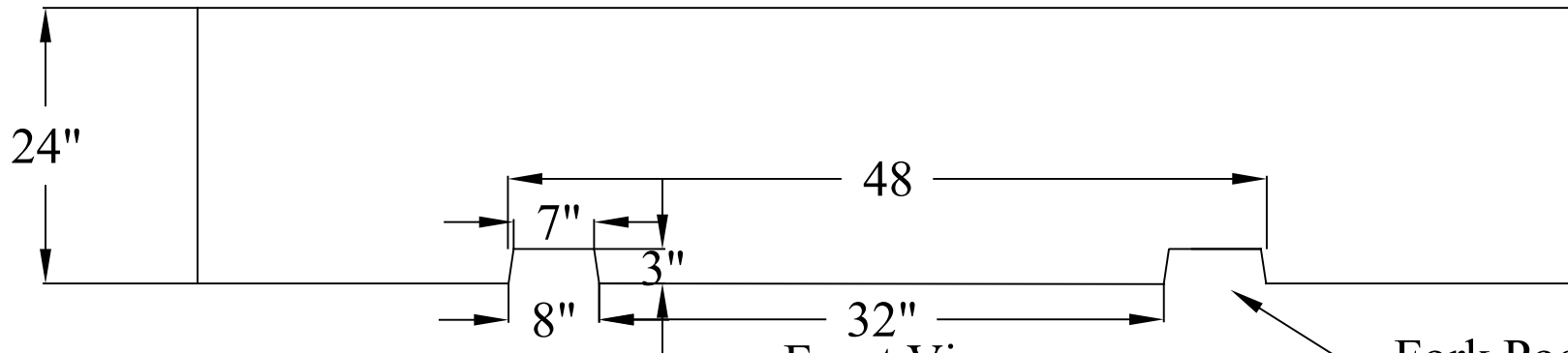
Front View
